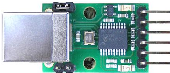
Bootloader Link - Fit link for Bootloader mode
