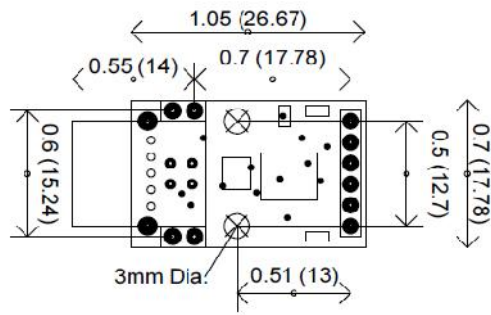
USB-ISS Mounting holes - Top View
