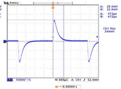
V_{inmax} , Full Load Transient Peak 240mV Transient Response 472µs
