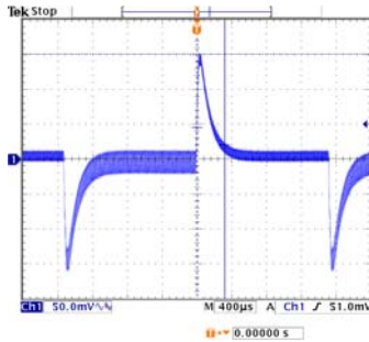
V_{inmin} , Full Load Transient Peak 152mV Transient Response 320µs
