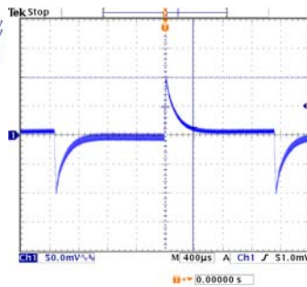
V_{innom} , Full Load Transient Peak 100mV Transient Response 384µs
