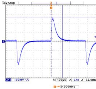
V_{inmin} , Full Load Transient Peak 270mV Transient Response 496µs
