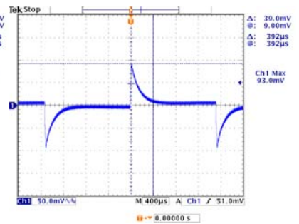
V_{inmax} , Full Load Transient Peak 93mV Transient Response 392µs
