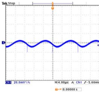
V_{inmin} , Full Load Output Ripple & Noise = 26.8mV
