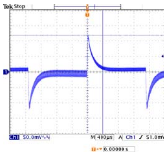
V_{inmin} , Full Load Transient Peak 119mV Transient Response 400µs
