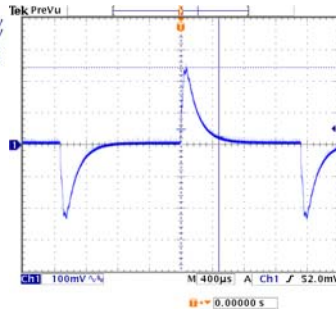
V_{innom} , Full Load Transient Peak 246mV Transient Response 480µs
