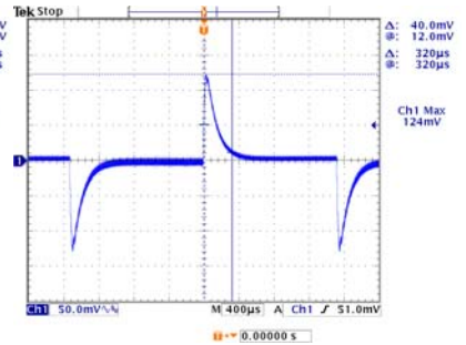
V_{inmax} , Full Load Transient Peak 124mV Transient Response 320µs
