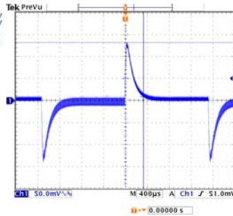
V_{innom} , Full Load Transient Peak 133mV Transient Response 328µs
