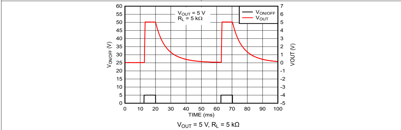
Figure 7-19. Turn-off Waveform (New Chip)
